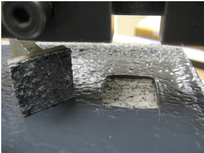
Photo No. 2 Pull-Off Strength - CMU Substrate Typical Condition After Testing
